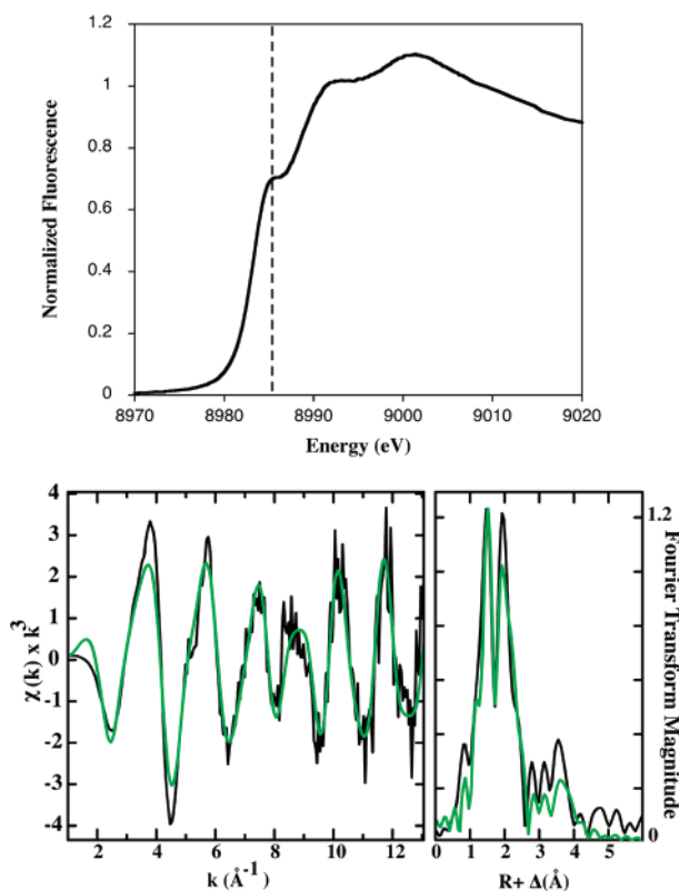
Figure 2. XAS analysis of Cu(II)-loaded methanobactin. Top: Cu XANES spectrum. Dashed line identifies the 1s \rightarrow 4p transition at 8985 eV. Bottom: EXAFS (left) and its Fourier transform (right). Raw data are shown in black with the best fit superimposed in green.
